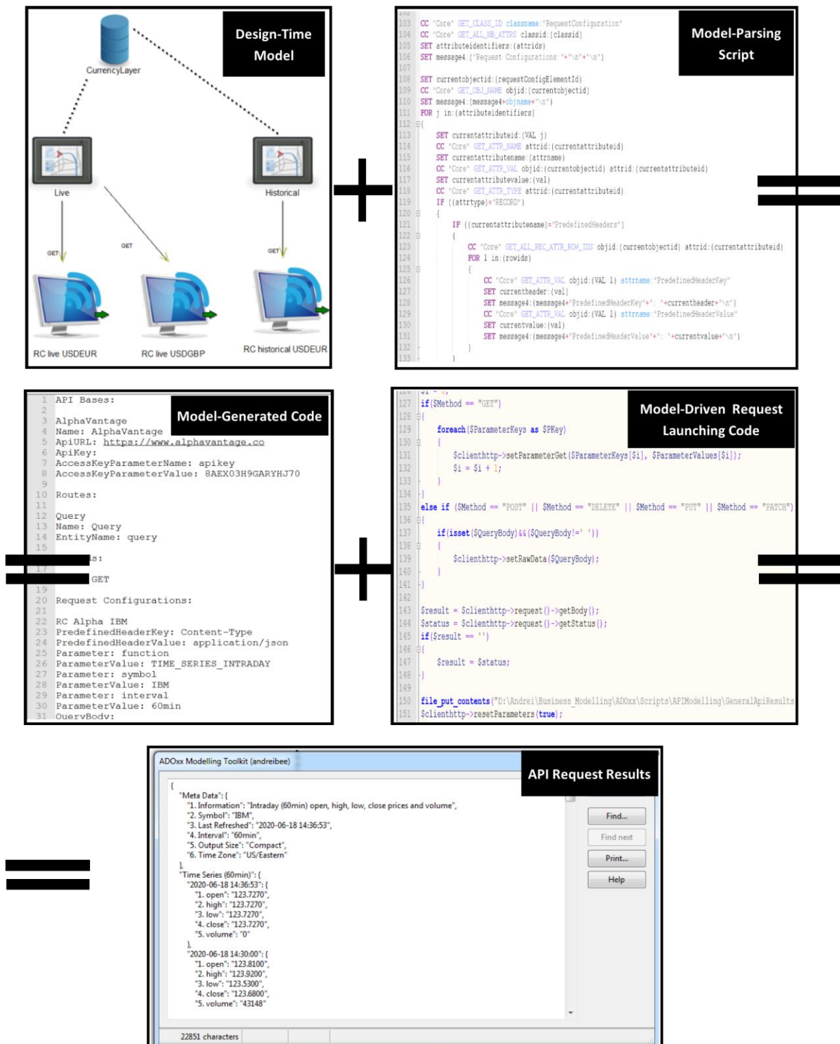
Figure 9. The model-driven API request execution cycle
